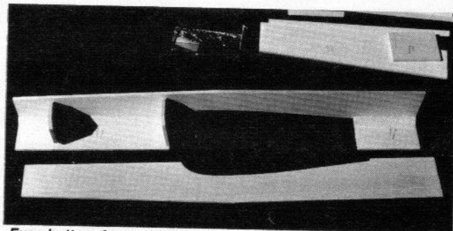
Fuse bottom front and rear in place. Right side, firewall, former and 1/2" triangle in place.
