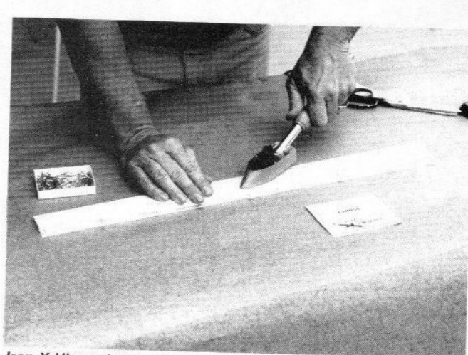
Iron X-Hinge down onto elevon.
